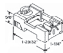
Pivot Lock Shoe ( White Cam )
