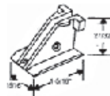
Carrier
