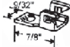
Metal Sash Clips
