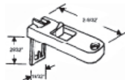
Tilt Window Slide Latch
