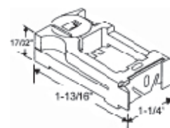
Pivot Lock Shoe ( Blue Cam )
