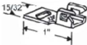
Metal Sash Clips
