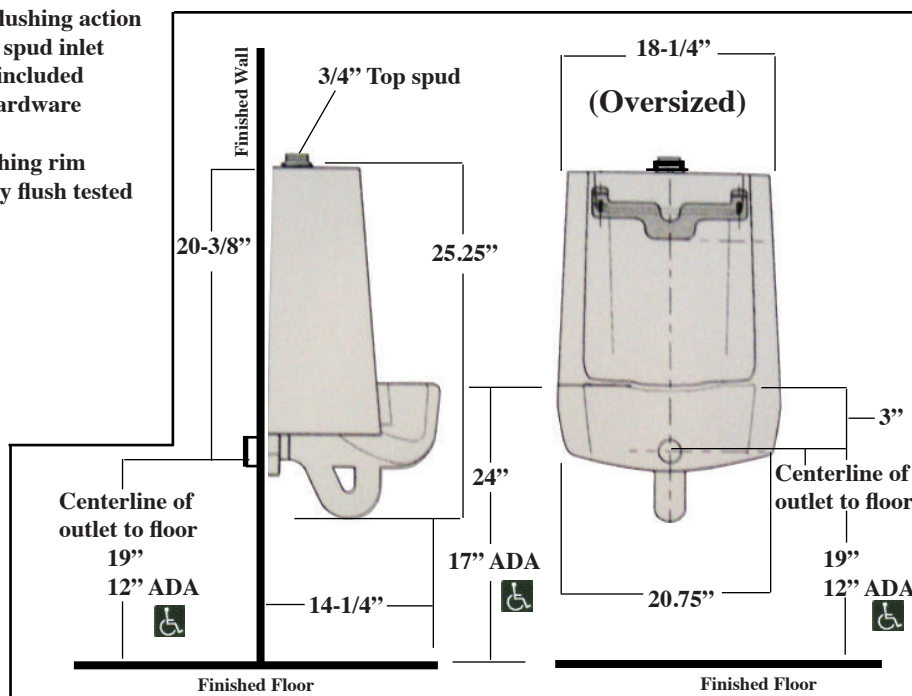
MODEL SU-1209 Vitreous China Top Spud Water Urinal
