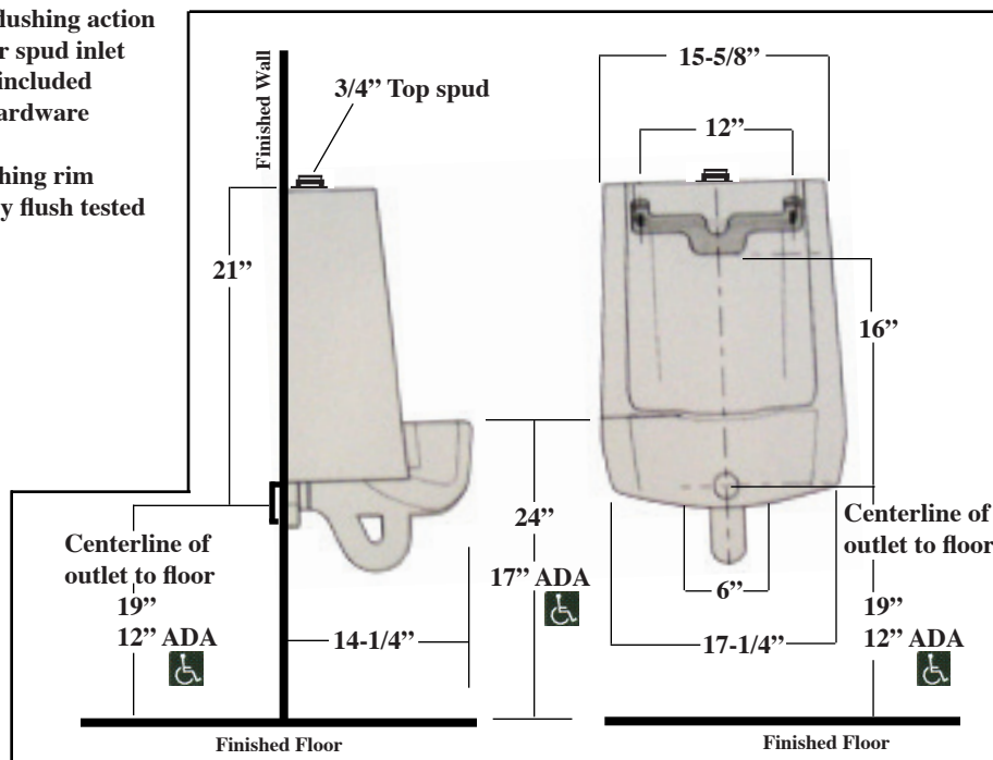
MODEL SU-1009-a Vitreous China Top Spud Water Urinal
